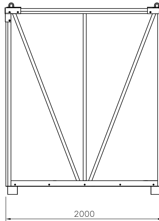
X1 Elevation
