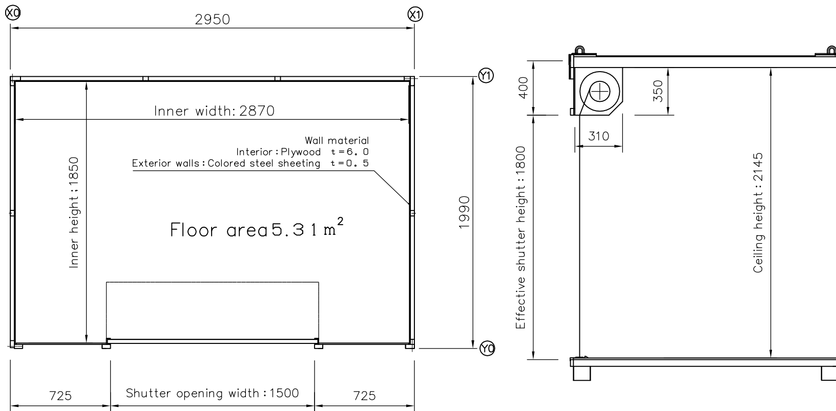
Floor plan
